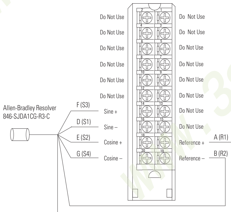
1756-PLS Resolver
