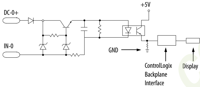
Simplified Schematic
