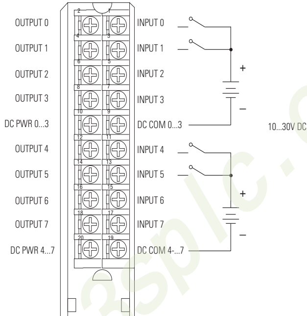
1756-PLS Inputs—Left Side
