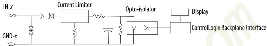
Simplified Schematic
