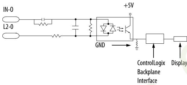
Simplified Schematic
