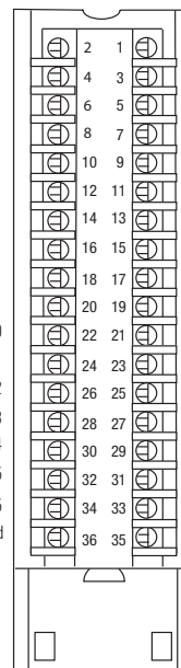
1756-IB16IF, 1756-IB16IFK
