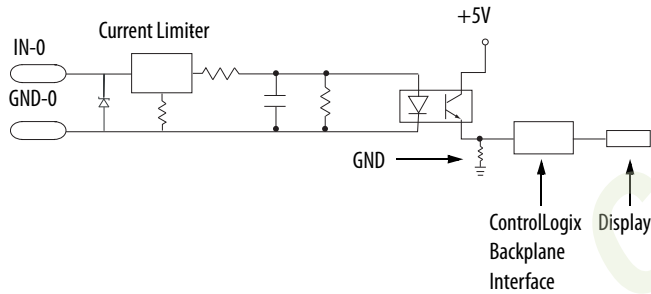
Simplified Schematic
