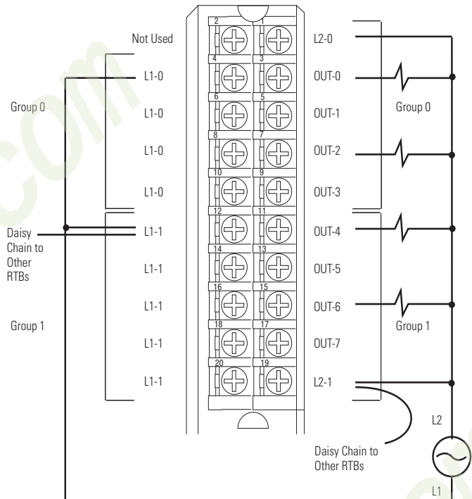
1756-0A8D
