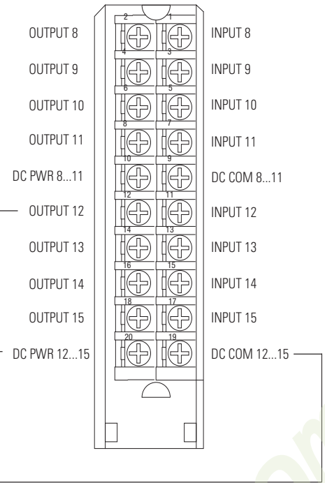
1756-PLS Outputs—Right Side
