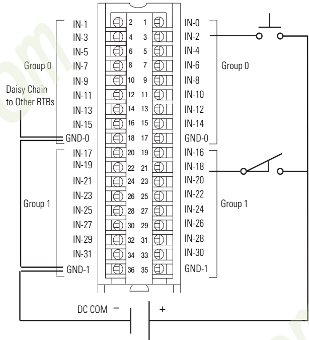
1756-IB32, 1756-IB32K
