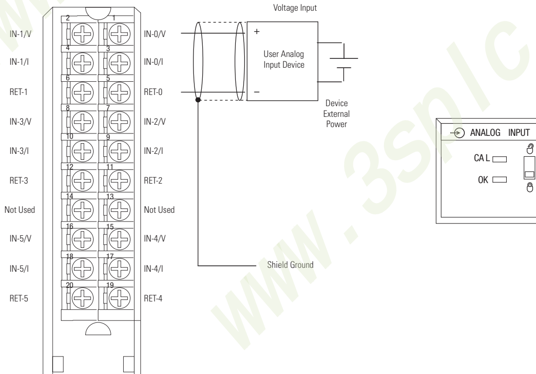
1756-IF6I Voltage
